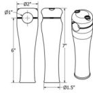
TC BROS. 6" BLACK SPRINGER RISERS FOR 1" DIAMETER HANDLEBARS TC Bros. SKU: 101-0226
