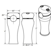
TC BROS. 4" CHROME SPRINGER RISERS FOR 1" DIAMETER HANDLEBARS TC Bros. 101-0223
